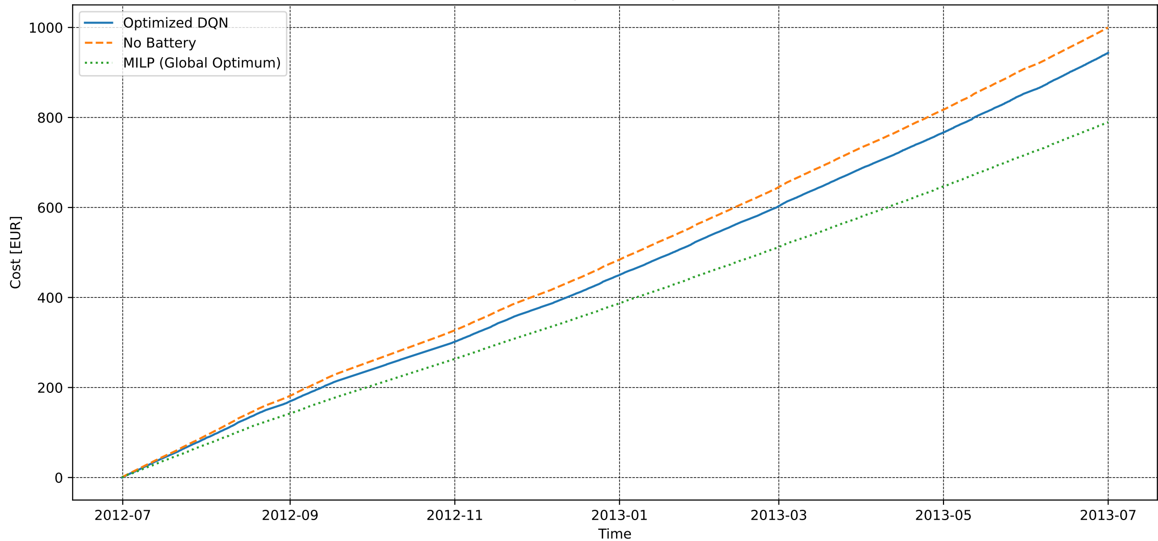
User 66 - Basic Training - Electricity Cost [DQN vs MILP]
